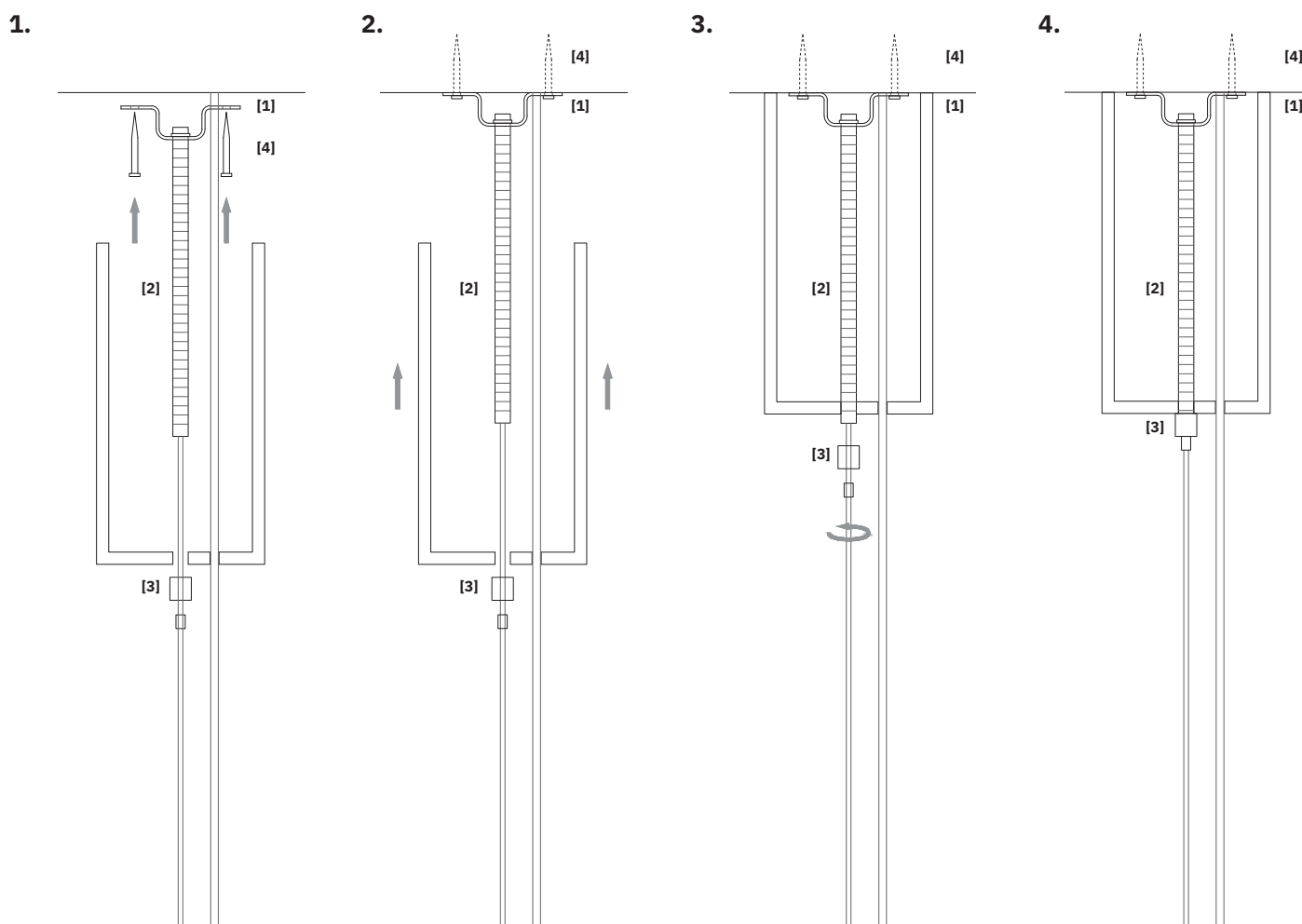
[1] Mounting element
